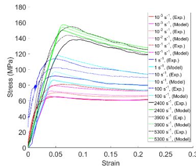
Fig. 2: Model predictions and experimental validation.
