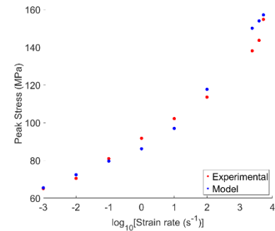
Fig. 3: Comparing peak stresses for model predictions and experiments.
